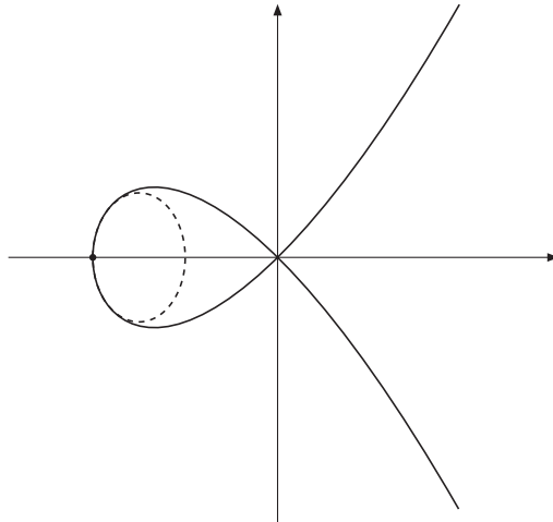
FIGURE 2. The nodal cubic from Example 2.3 with the hyperosculating conic O_{p_2} at the sextactic point p_2 .
