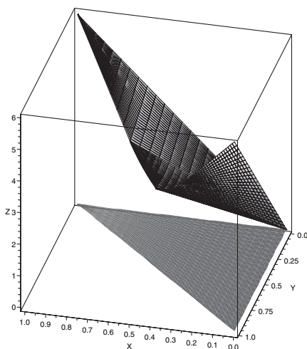
FIGURE 2. \Psi_{\Delta}(x, y) on the simplex.
