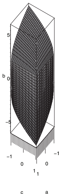
FIGURE 1. Unit ball of (\mathbb{R}^3, \|\cdot\|_\Delta) .
